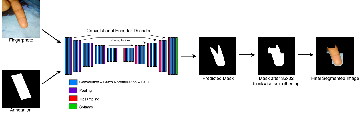
Figure 5: Stepwise illustration of the segmentation framework using VGG SegNet followed by 32 \times 32 block-wise smoothing.
