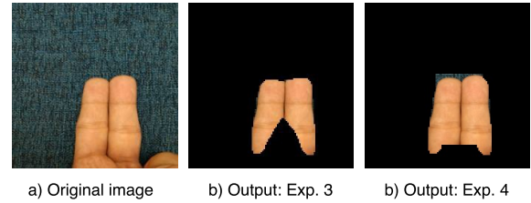
Figure 9: Sample showing the significance of 32×32 block-wise smoothing post VGG SegNet.
