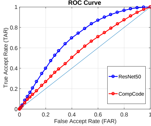
Figure 10: ROC curve for the proposed segmentation with ResNet50 and CompCode features on the UNFIT database.
