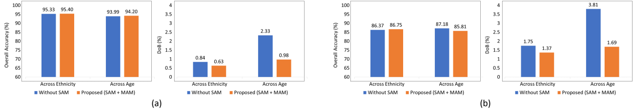
Figure 8. Classification accuracy and DoB (%) by ablating the Sensitive Attention Module (SAM) and the sub-network for sensitive attribute prediction corresponding to the (a) MORPH and (b) UTKFace datasets. Comparison is performed with the proposed Attention Aware Debiasing (AAD) method.
