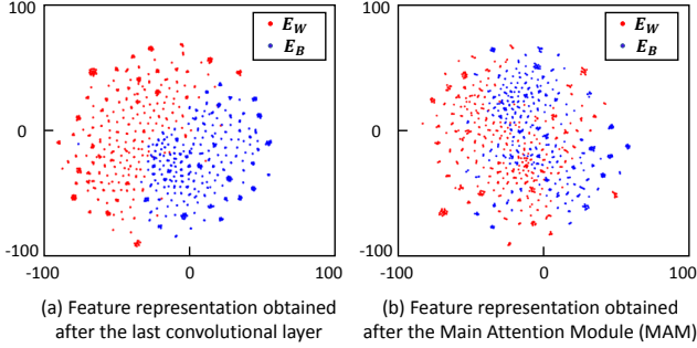
Figure 6. t-SNE visualizations of the 256-dimensional feature representation of the testing set corresponding to the MORPH dataset for gender prediction. (a) Shows the visualization of the feature representation obtained after the last convolutional layer of the model. (b) Shows the visualization of the updated feature representation obtained after the attention modules corresponding to the model trained using the proposed AAD method to unlearn the ethnicity-related features during gender prediction.
