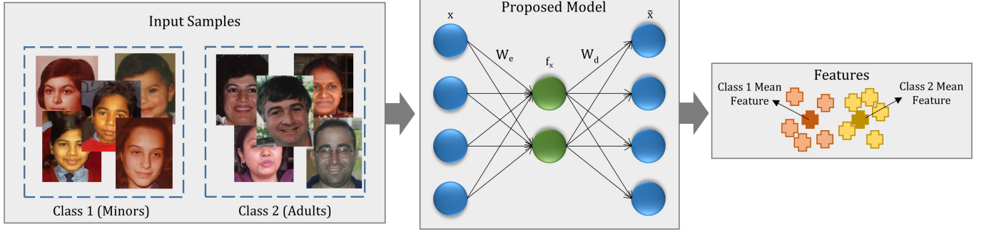
Fig. 5. Proposed Class Specific Mean Autoencoder. x and \hat{x} represent the input and the reconstructed samples respectively, W_e and W_d denote the encoding and decoding weights, and f_x corresponds to the learned feature vector.
